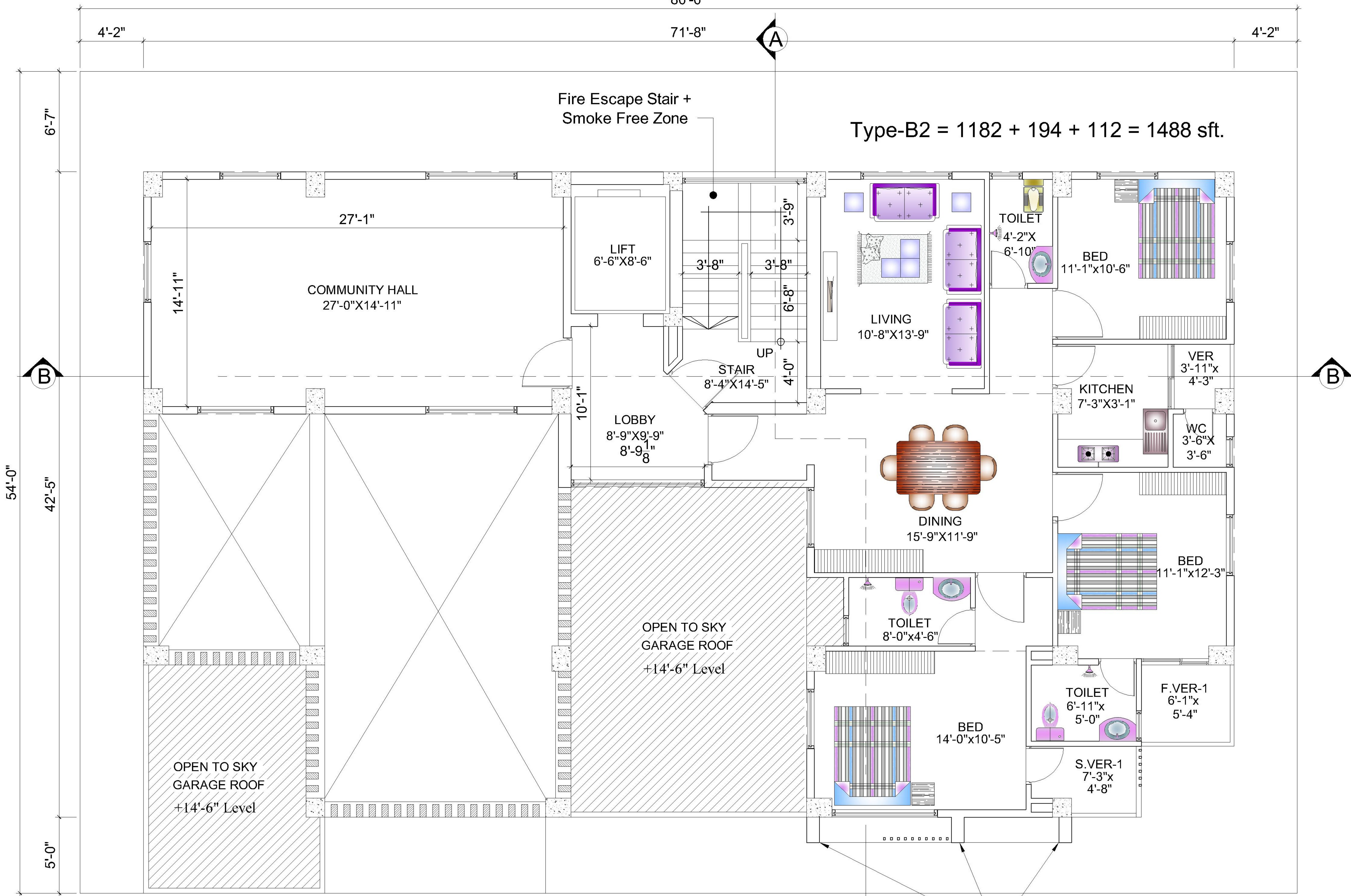
1ST. FLOOR PLAN
