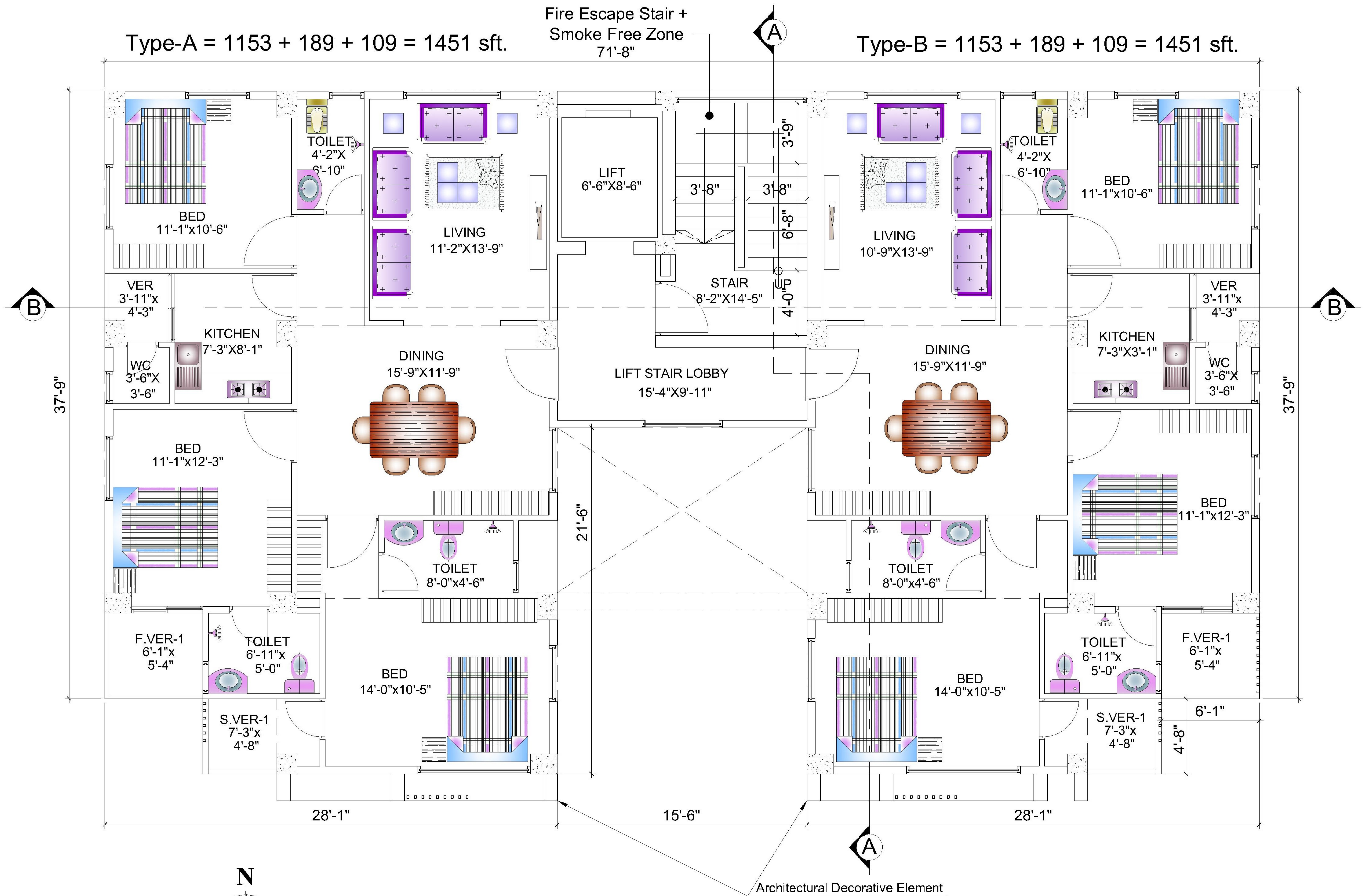
2ND. FLOOR PLAN
